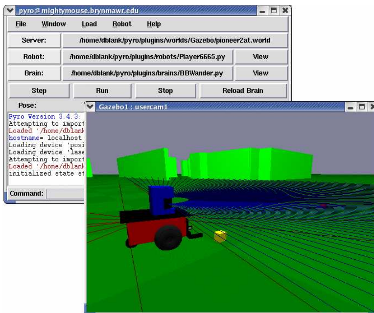
Figure 1: A view of Pyro controlling a Pioneer robot in the Gazebo simulator.
