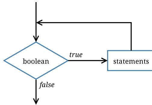
Figure 7.1: Flow of execution for a while loop.
