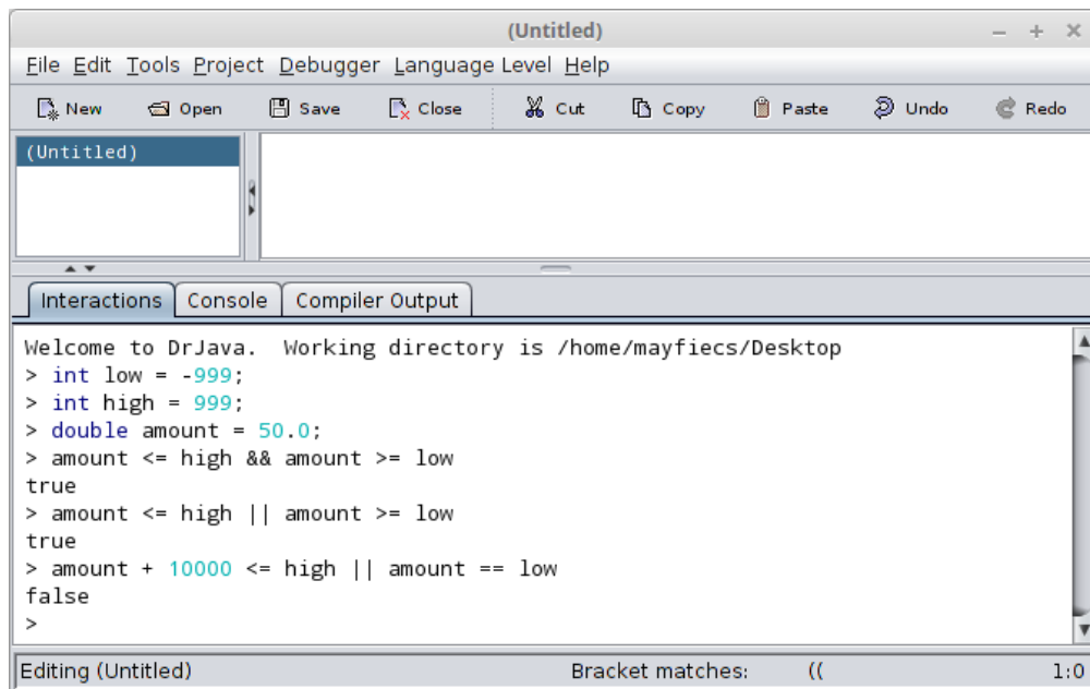
Figure A.2: The Interactions pane in DrJava.
