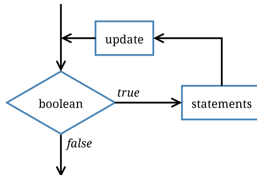
Figure 7.2: Flow of execution for a for loop.
