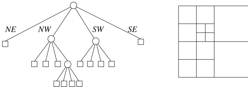
Figure 4: Quadtree
